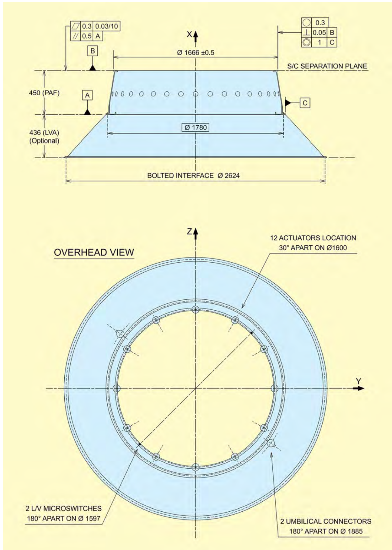
Figure A10.2 – PAS 1666MVS – General view
