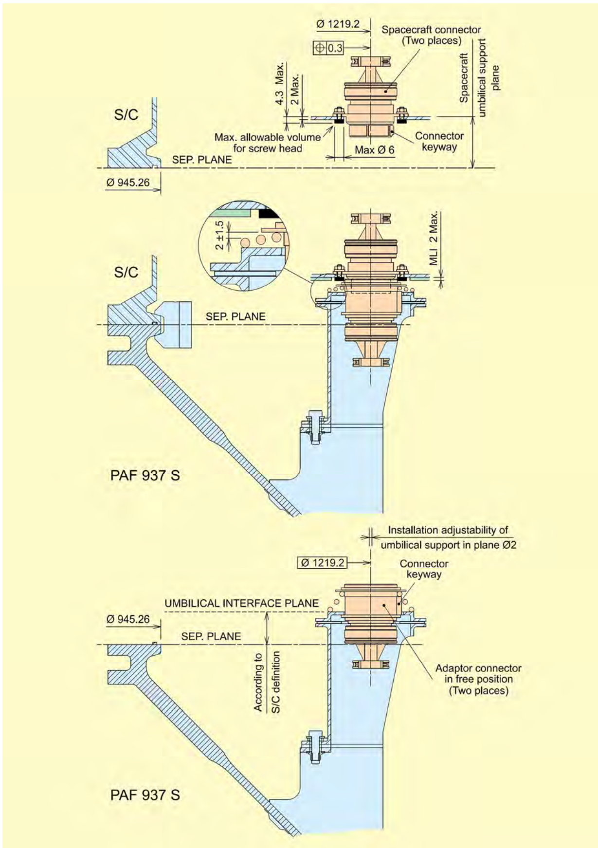
Figure A7.5 – PAS 937S – Umbilical connectors
