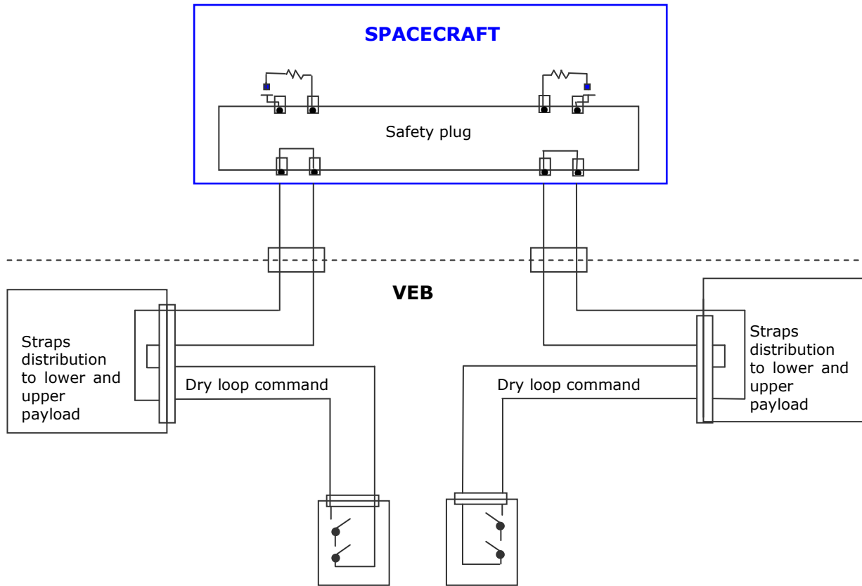
Figure 5.5.2.1.a - Dry loop command diagram
