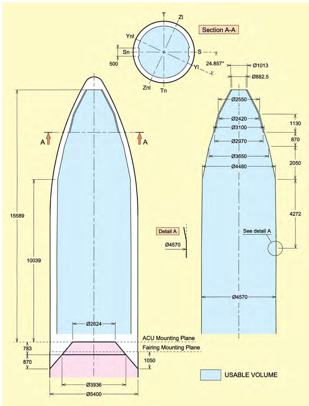
Figure A5.1 – Usable volume beneath the payload fairing
