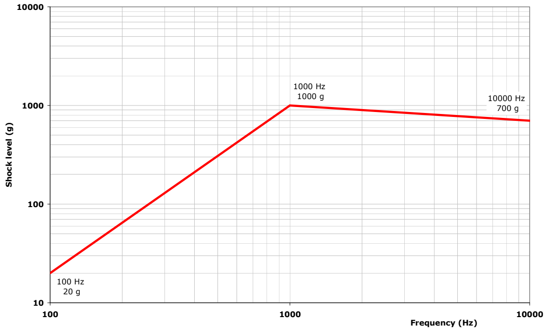
Figure 3.2.6.a Envelope shock spectrum for clampband release at spacecraft interface and for fairing and L/V stage separation events
