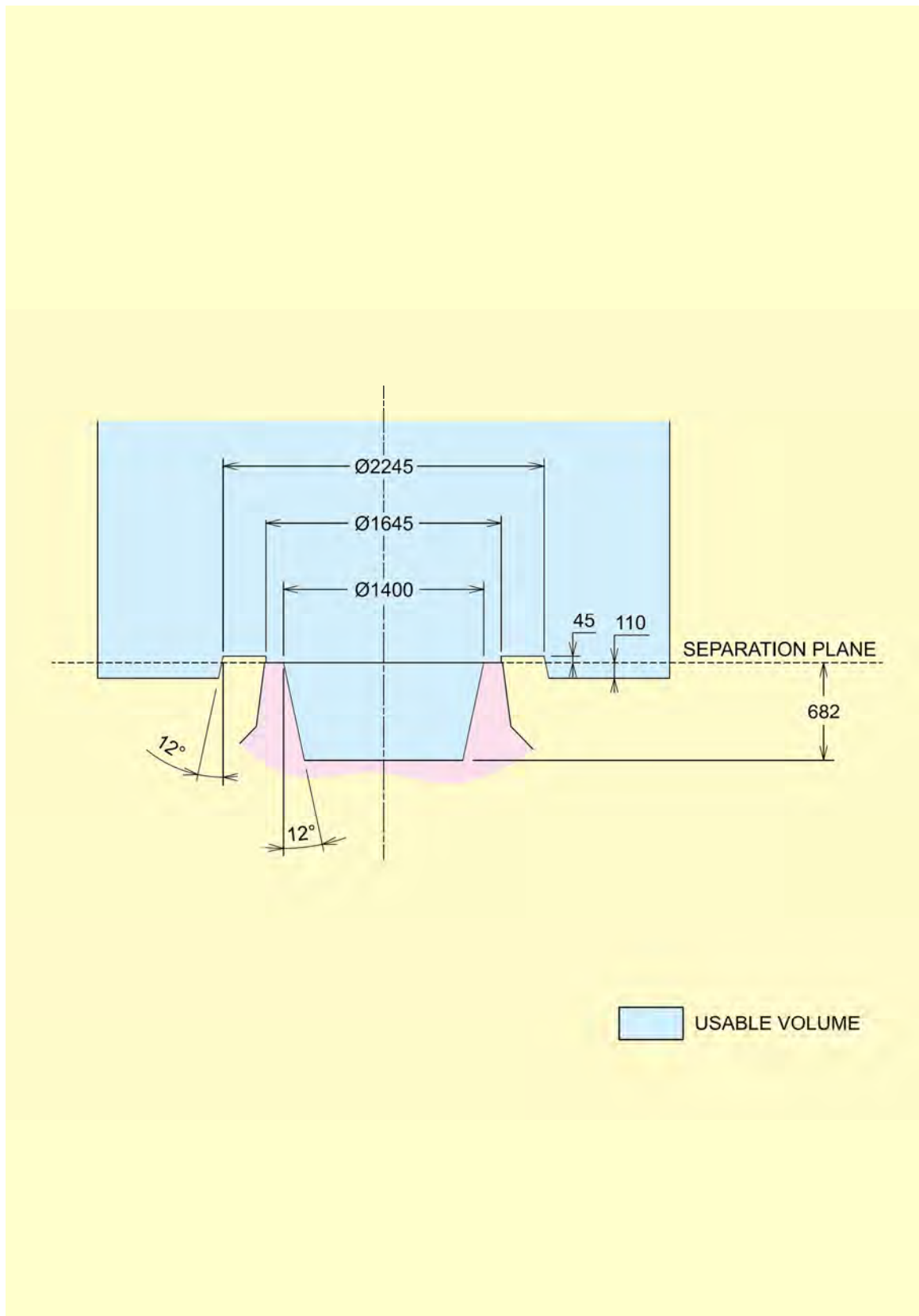
Figure A11.7 – PAS 1666S – Usable volume
