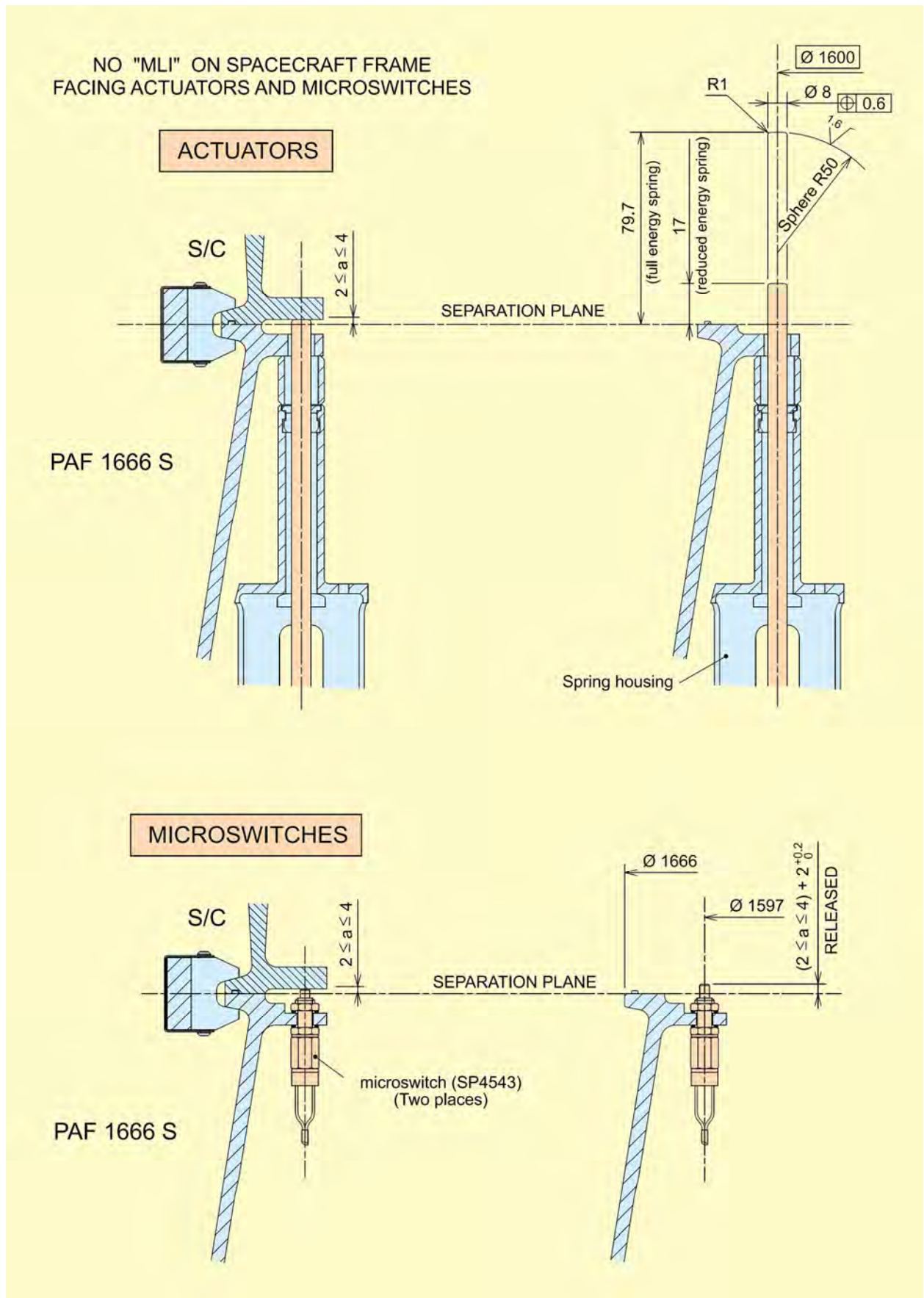
Figure A11.4 – PAS 1666S – Actuators and microswitches
