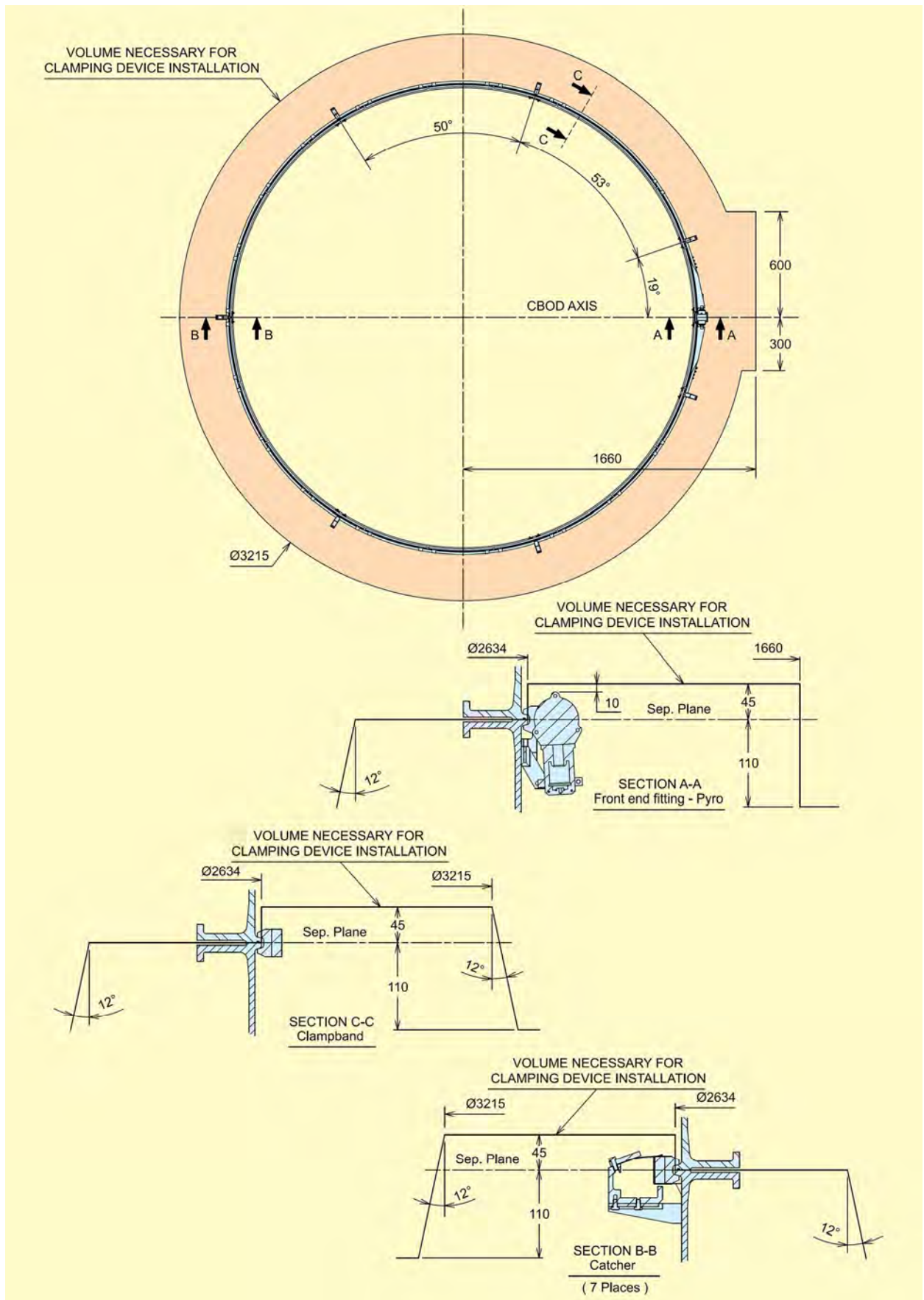
Figure A12.6 – PAS 2624VS – Clamping device interface
