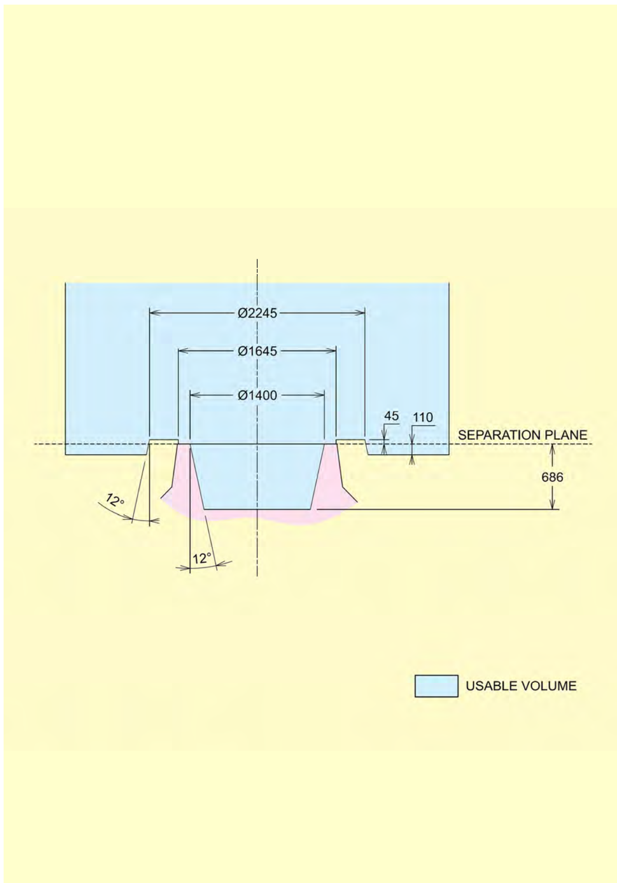
Figure A10.7 – PAS 1666MVS – Usable volume
