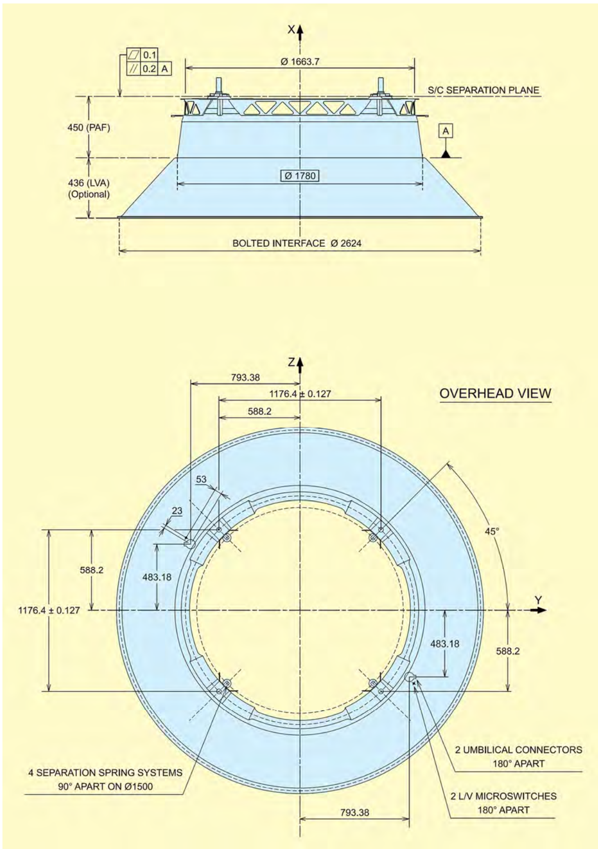
Figure A9.1 – PAS 1663 – General view
