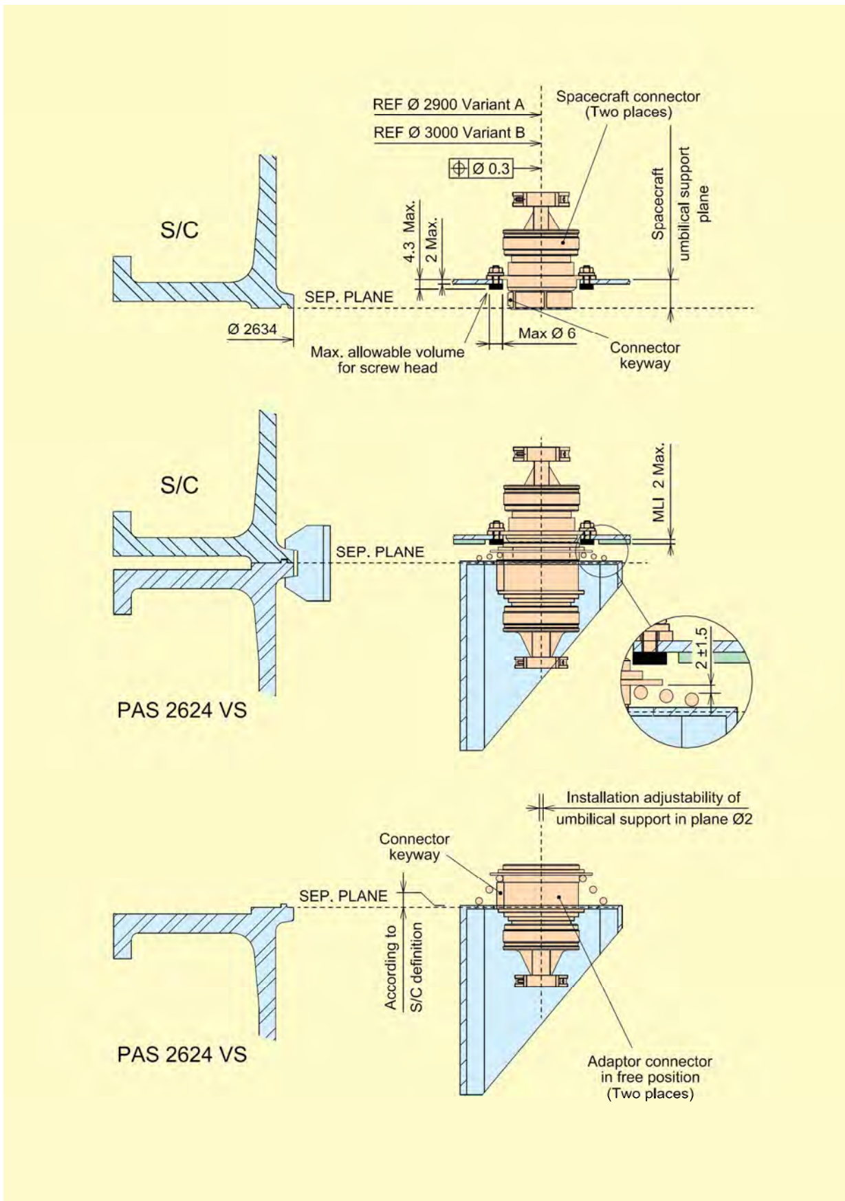
Figure A12.5 – PAS 2624VS – Umbilical connectors
