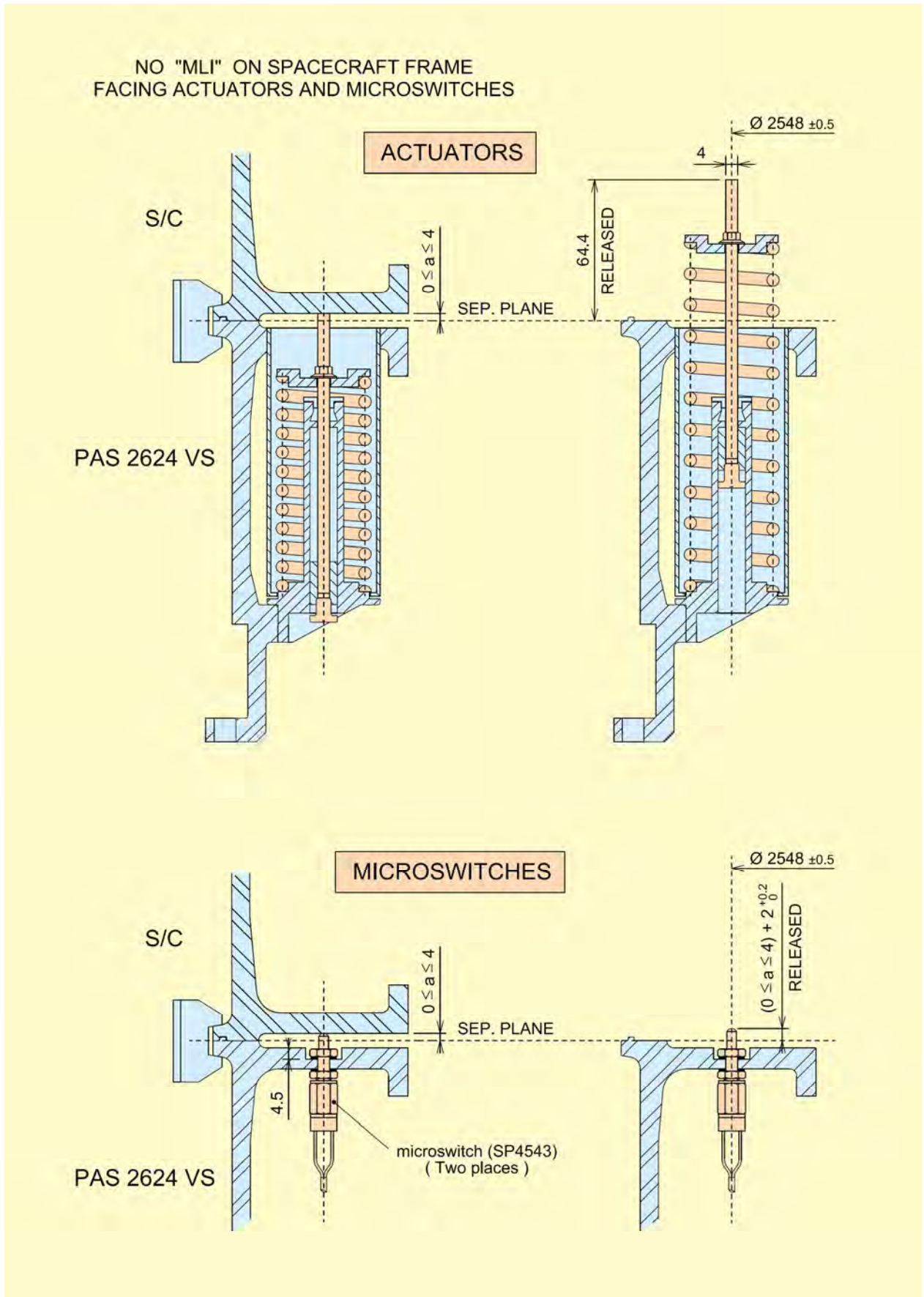
Figure A12.4 – PAS 2624VS - Actuators and Microswitches
