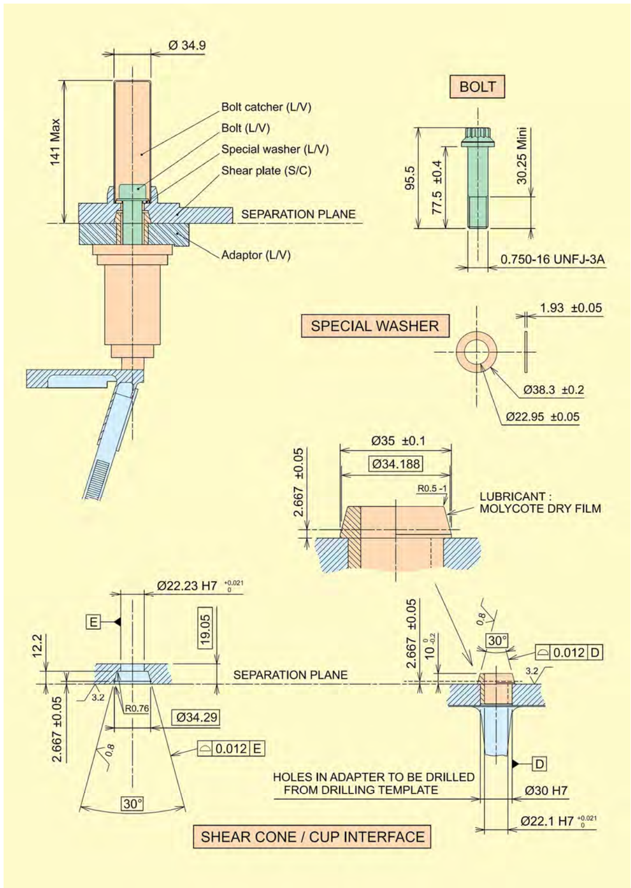
Figure A9.2 – PAS 1663 – Separation Subsystem
