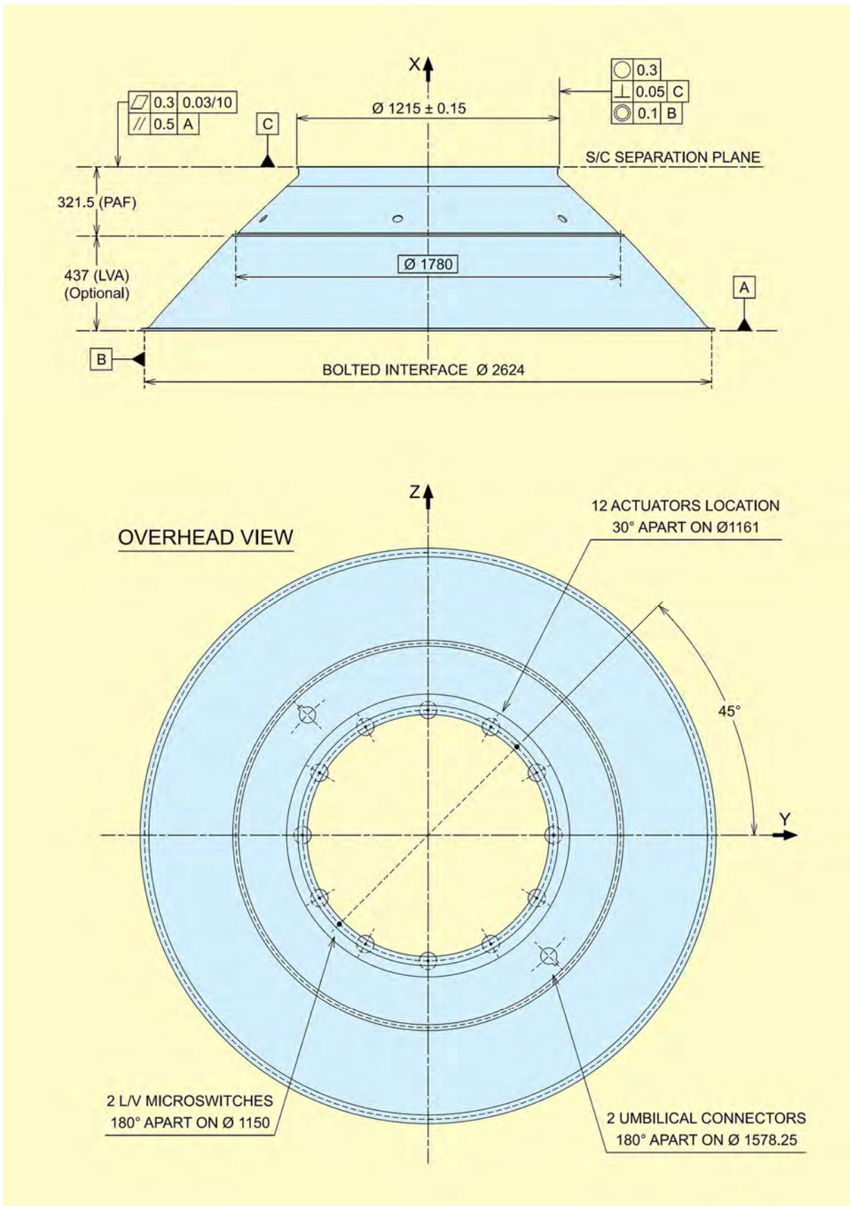
Figure A8.8 – PAS 1194C Variant A– General view
