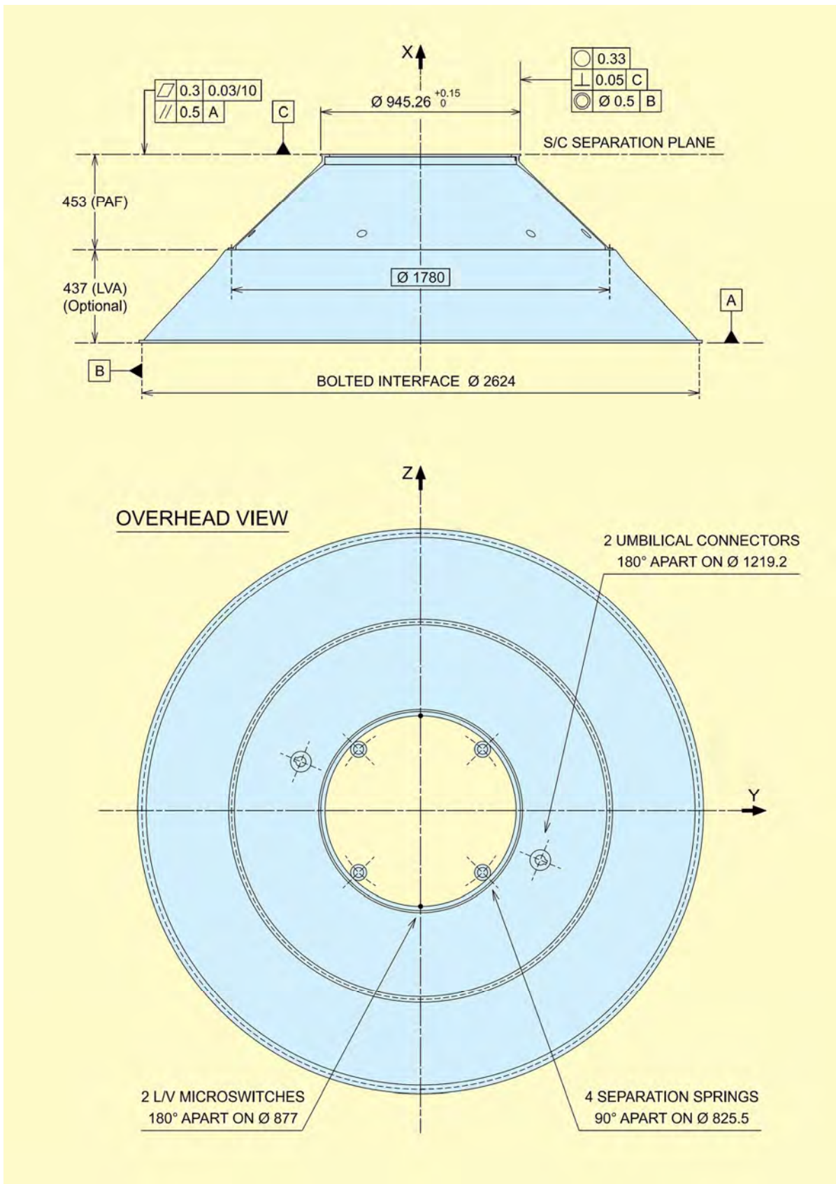
Figure A7.8 – PAS 937C Variant A – General view
