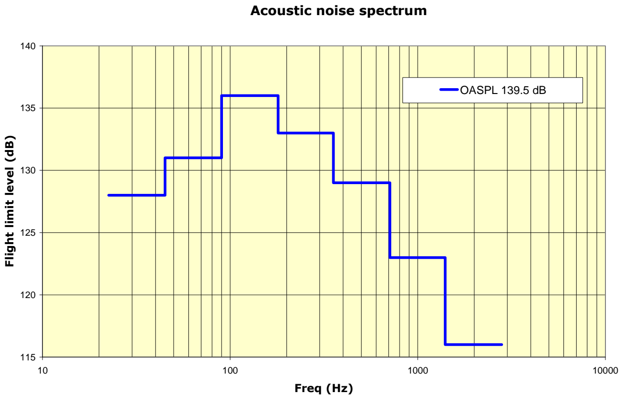
Figure 3.2.5.2.b - Acoustic noise spectrum
