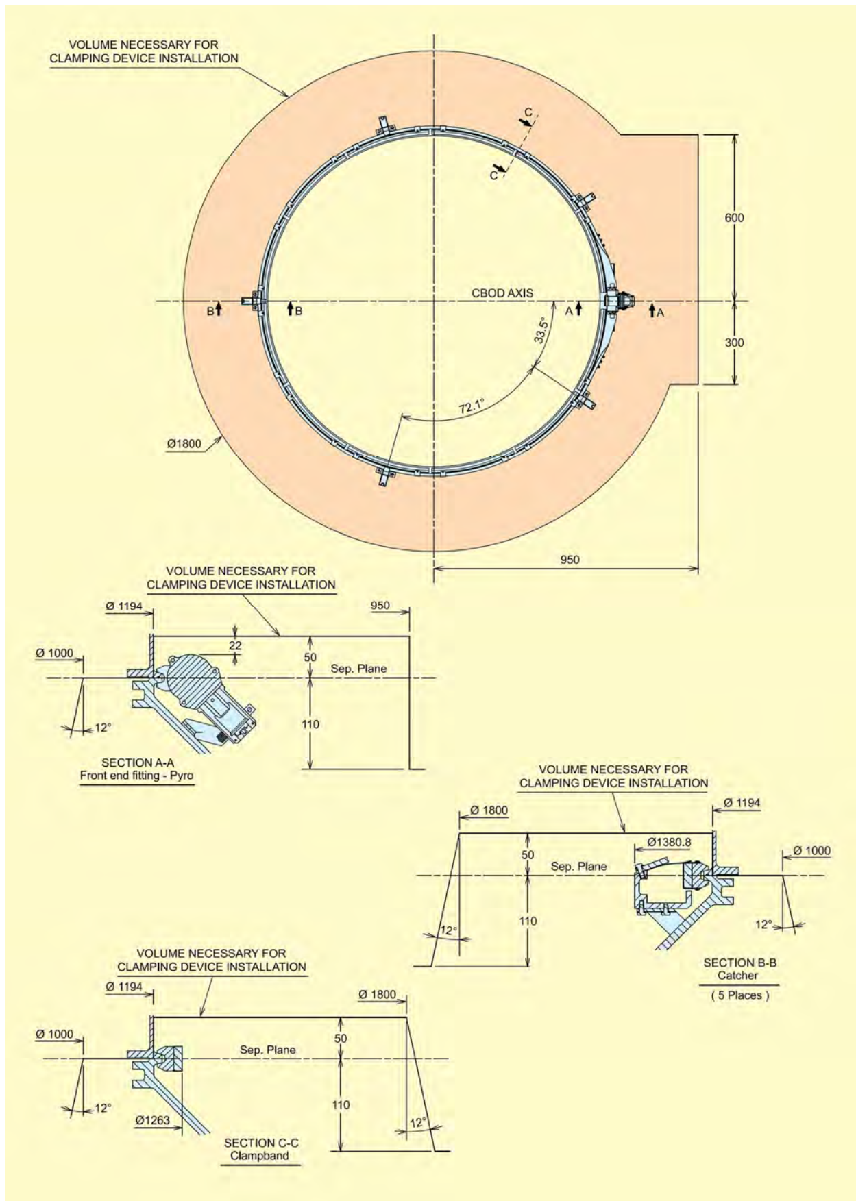
Figure A8.6 – PAS 1194VS – Clamping device interface
