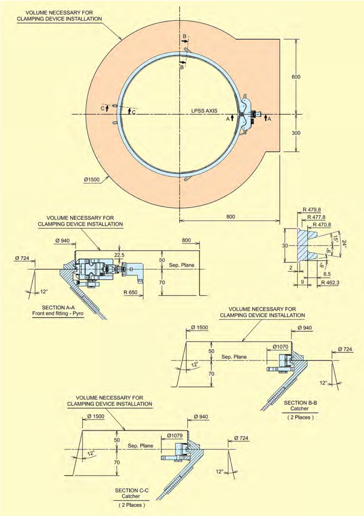
Figure A7.12 – PAS 937C – Clamping device interface
