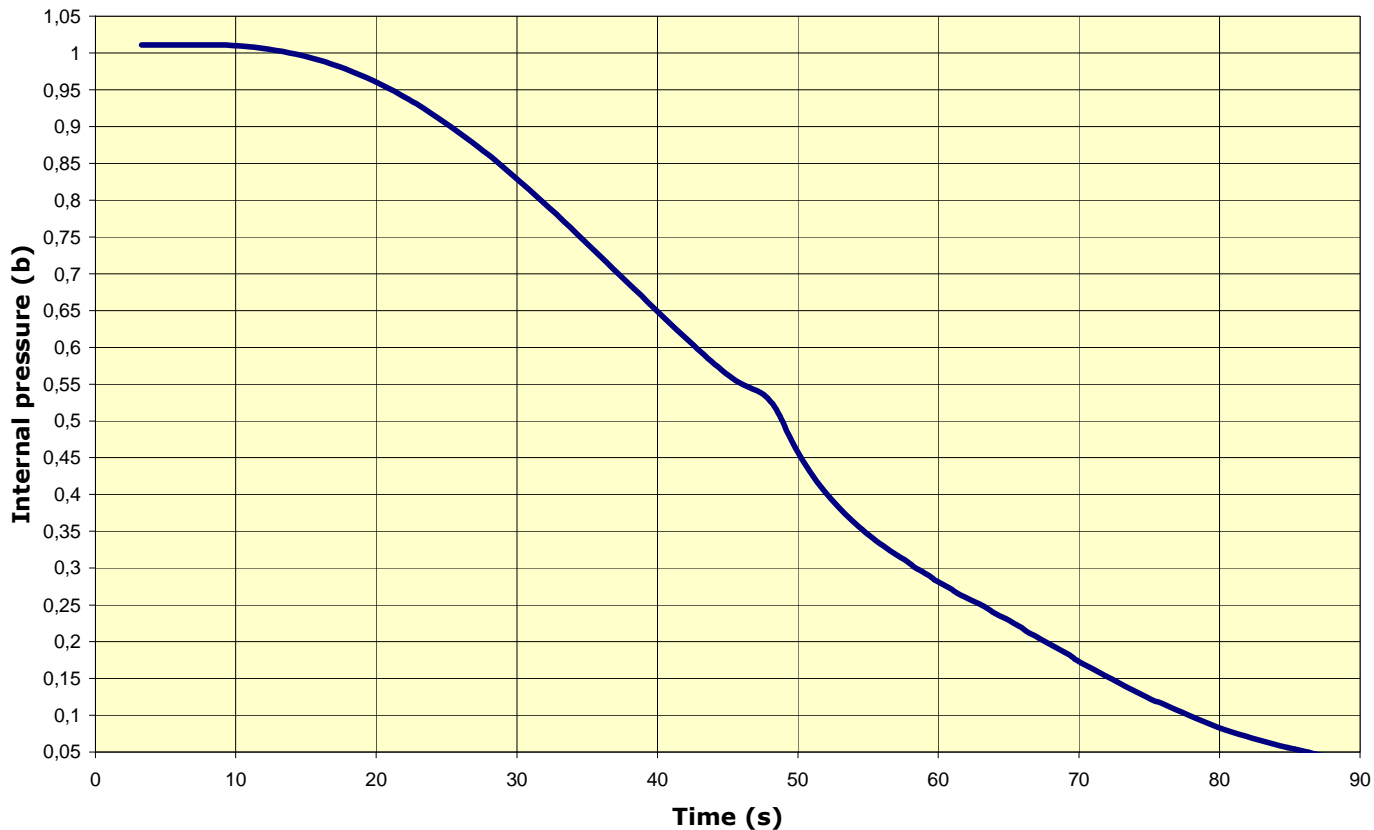
Figure 3.2.7.2.a – Variation of static pressure within payload volume
