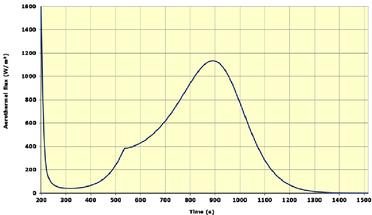
Figure 3.3.3.2.a – Aerothermal fluxes on trajectory Ariane 5 equipped with cryogenic upper stage (ESC-A) Fairing jettisoning constrained at 1135 W/m^2
