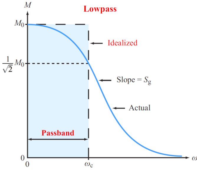
(a) Lowpass filter
