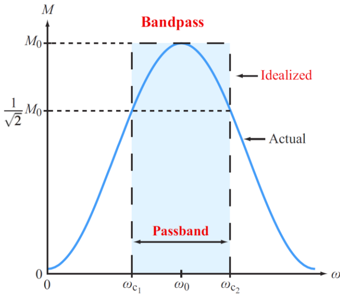
(c) Bandpass filter
